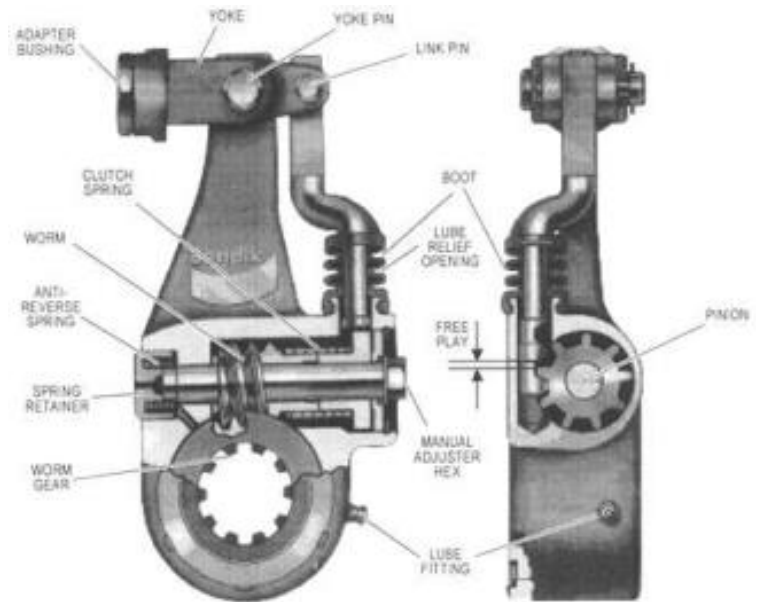
Automatic Slack Adjuster
