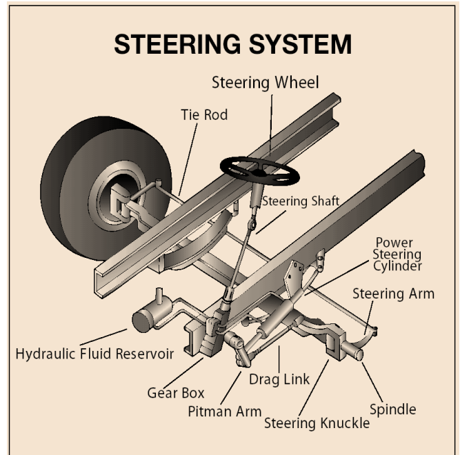
Figure 2.1 illustrates a typical steering system
