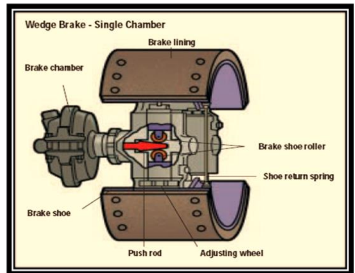
Figure 5.2a Wedge Brake
