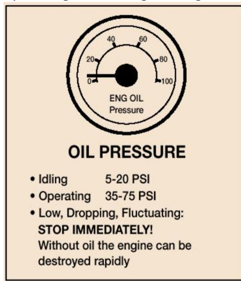
Figure 2.5 Oil Pressure
