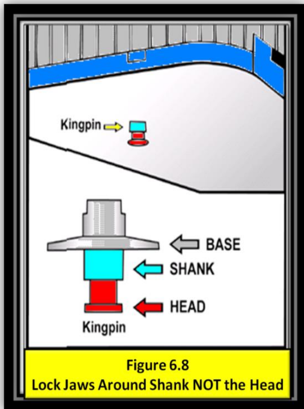
Figure 6.8 Kingpin
