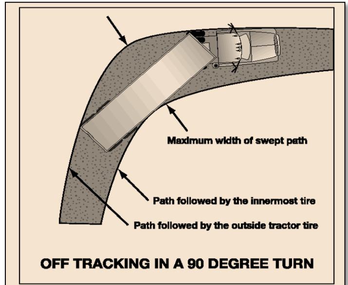
Figure 6.3 Offtracking
