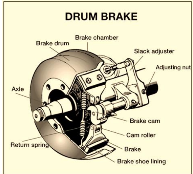
Figure 5.2 Drum Brake
