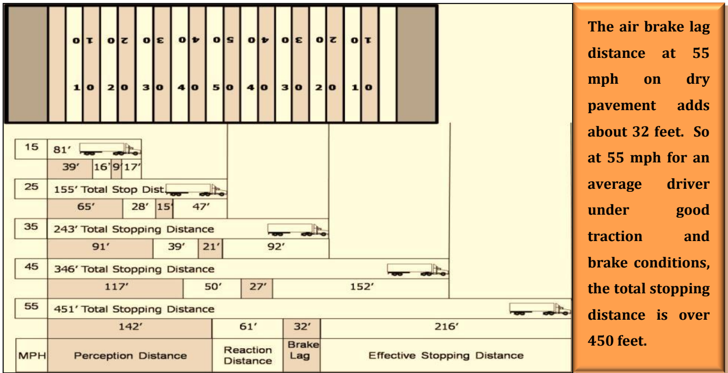
Figure 5.6 Stopping Distance
