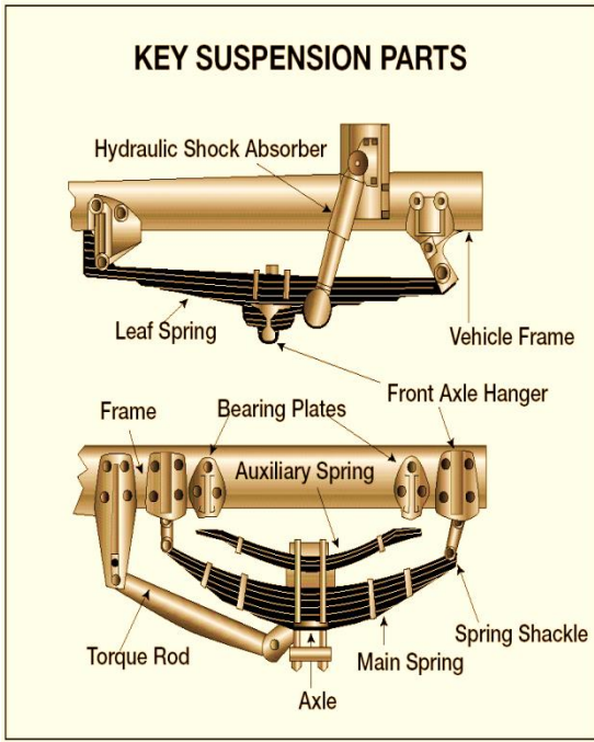
Figure 2.2 Key Suspension Parts
