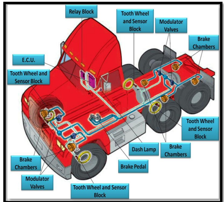
Figure 5.4 ABS System
