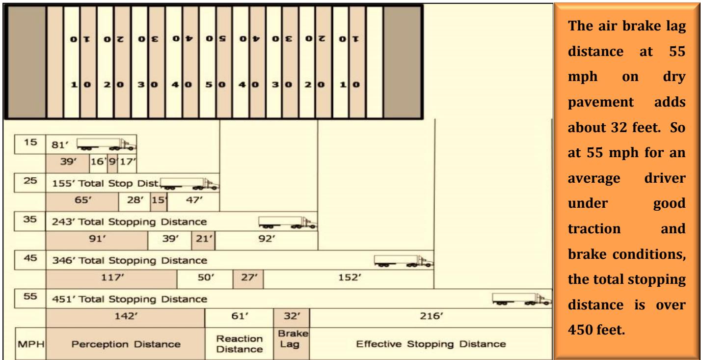
Figure 5.6 Stopping Distance
