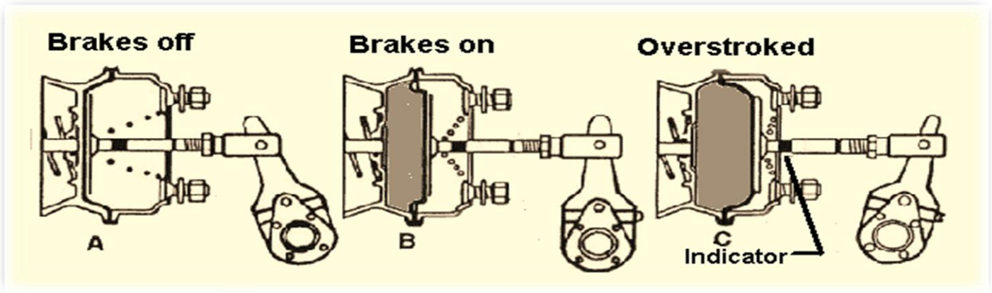
Figure 11.1 - Air Brake Adjustment
