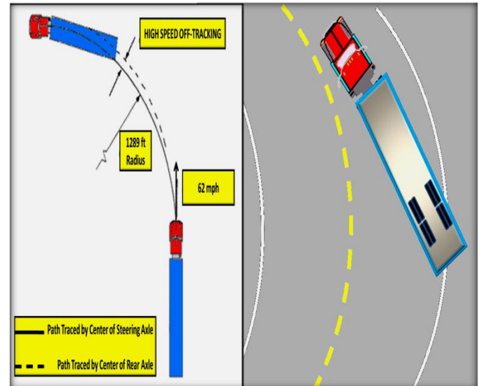
Figure 6.3A High-Speed Off-tracking
