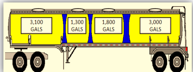
Fuel Trailer with bulkheads can carry different grades of fuel
